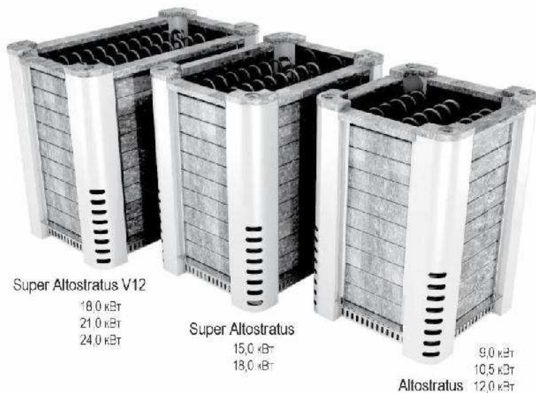
Altostratus
